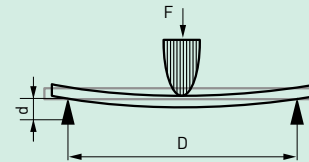
5.53-1 Flexion 3 points
