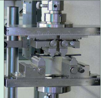
5.53-1 Flexion 3 points
