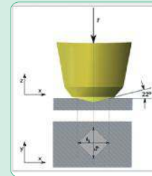
5.56-2 Essai Vickers
