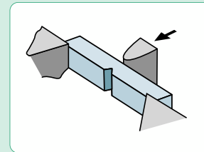
5.55-6 Charpy
