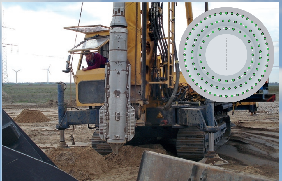
Vibro Compaction
